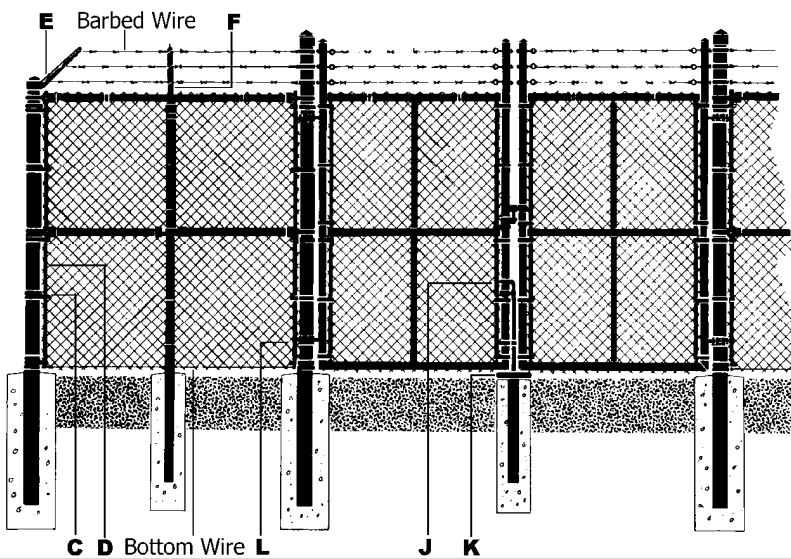
Double Gate – With 3 strands of barbed wire
